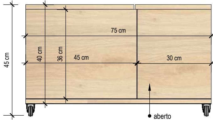
Vista frontal
