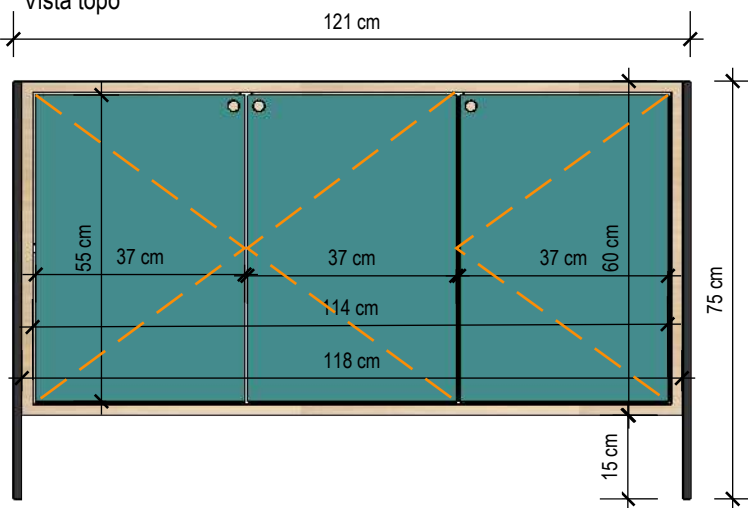
Vista frontal
