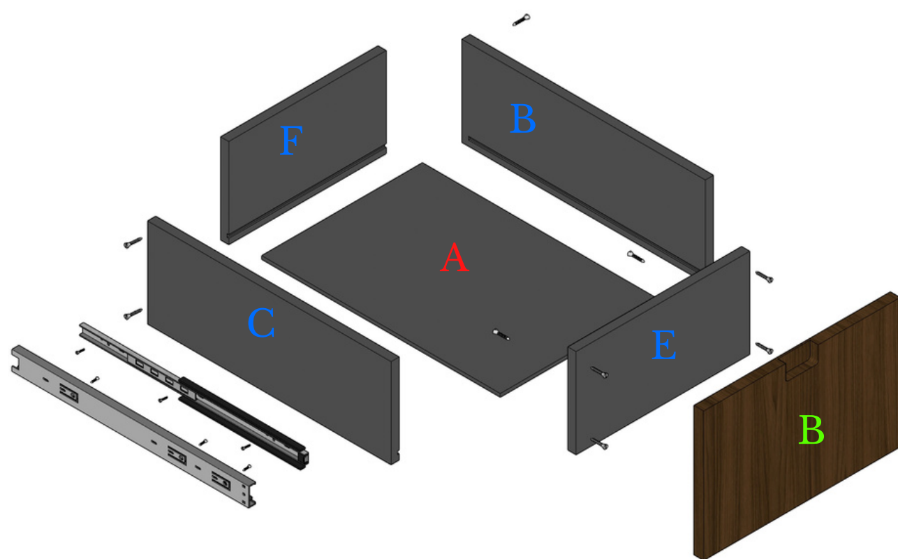
GAVETA EXPLODIDA
