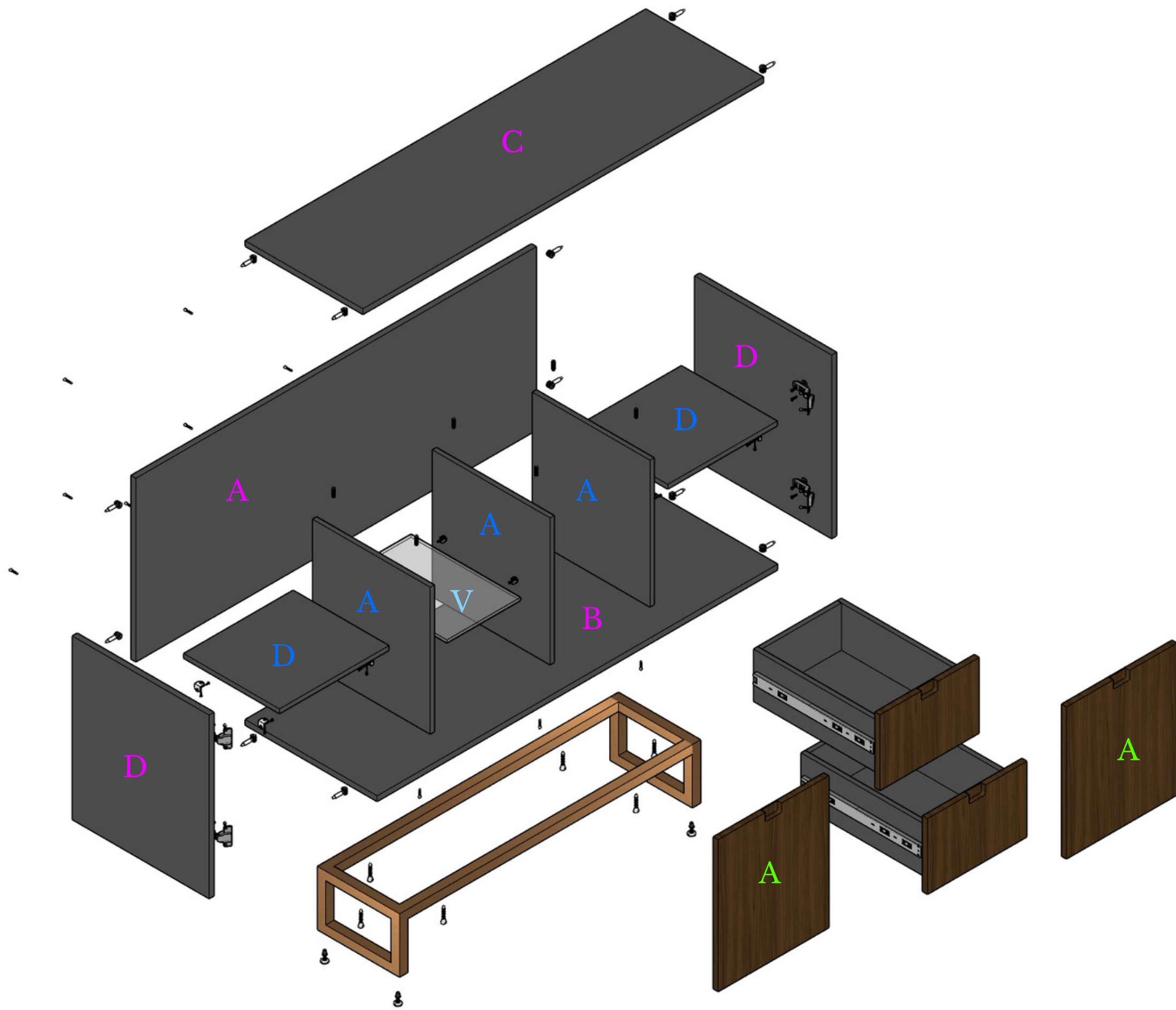
VISTA EXPLODIDA
